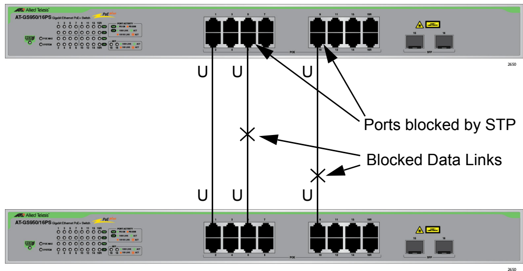
Figure 19. STP and VLAN Fragmentation with Untagged Ports
